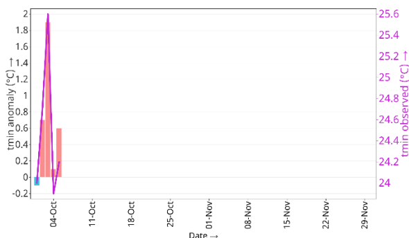
Minimum Temperature at Biratnagar Airport
