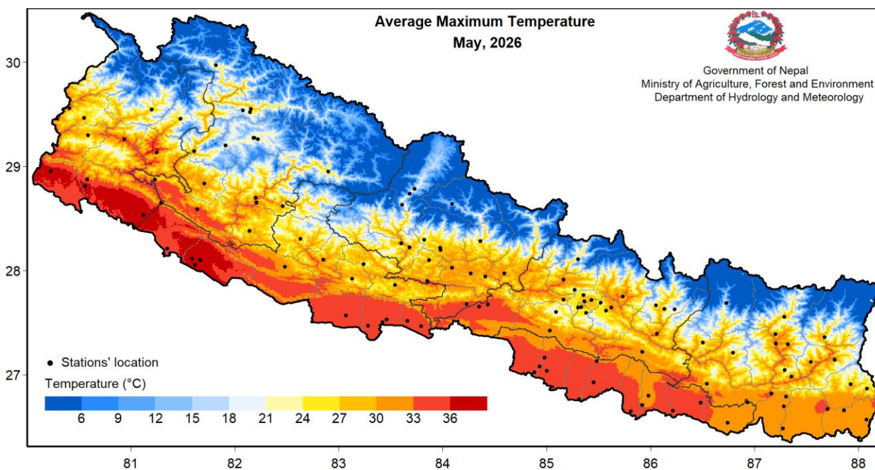
Figure 6: Maximum Temperature in May 2026
