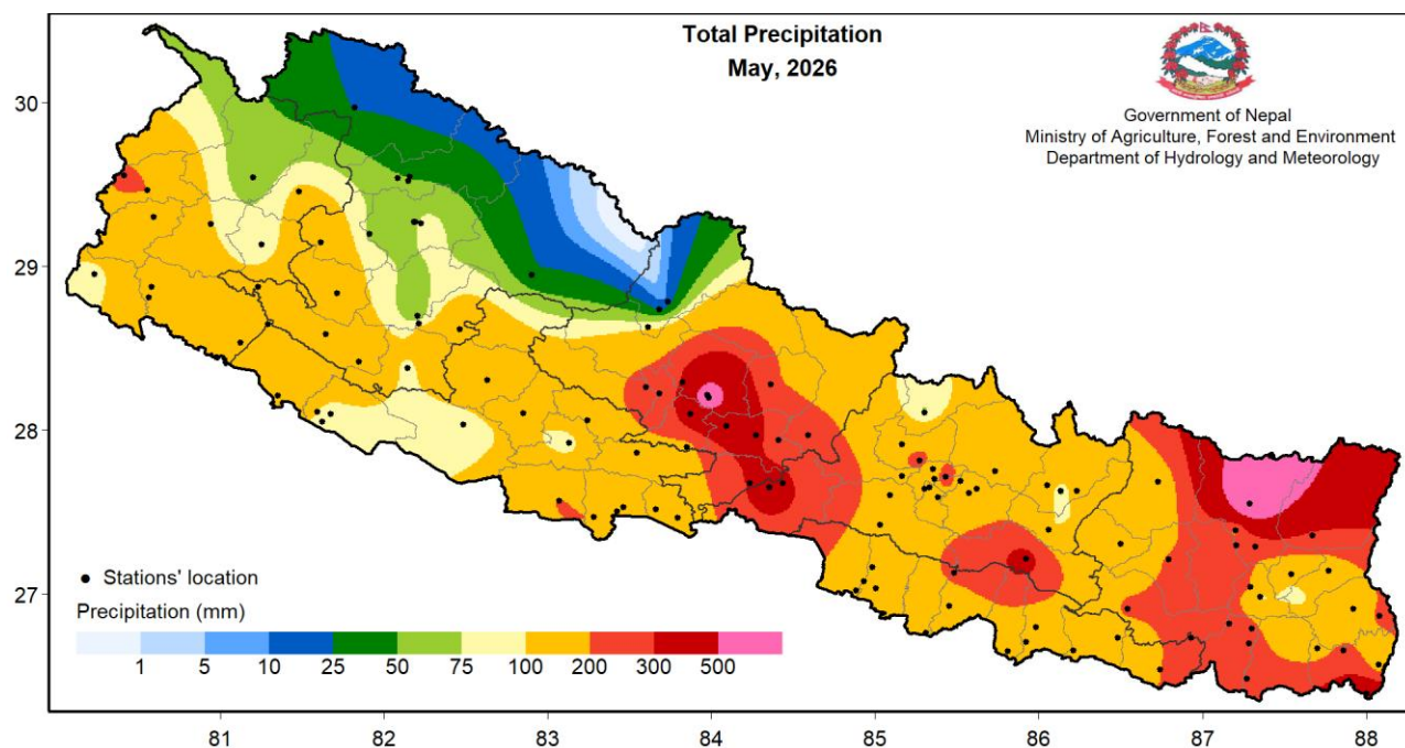
Figure 1 Total precipitation in May 2026
