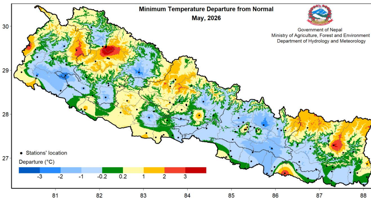
Figure 10: Departure from normal minimum temperature in May 2026
