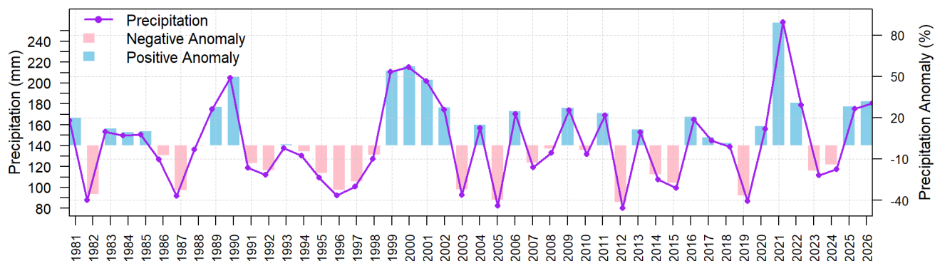
Figure 5: All Nepal monthly total precipitation of May from 1981 to 2026 (average of 104 stations)
