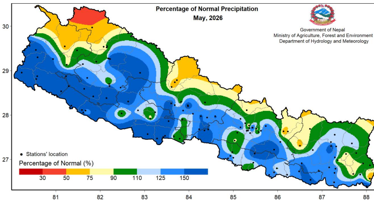
Figure 2: Percentage of normal precipitation in May 2026
