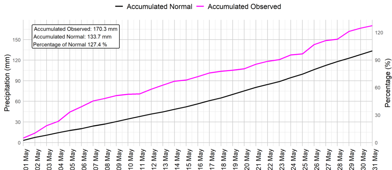
Figure 4: Cumulative average of daily normal and observed precipitation during May 2026
