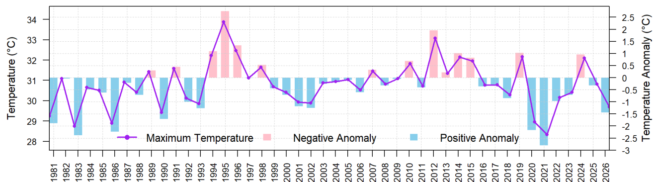
Figure 8: Monthly average maximum temperature anomaly of May from 1981 to 2026 of 66 stations (average of monthly average maximum temperature at stations having long term data)
