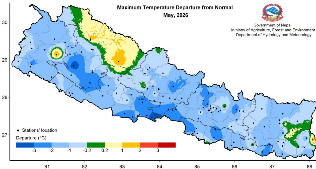
Figure 7: Departure from normal maximum temperature in May 2026
