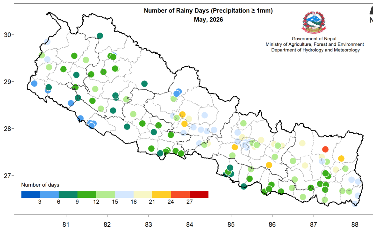
Figure 3: Number of Rainy days ( \geq 1 mm) during May 2026
