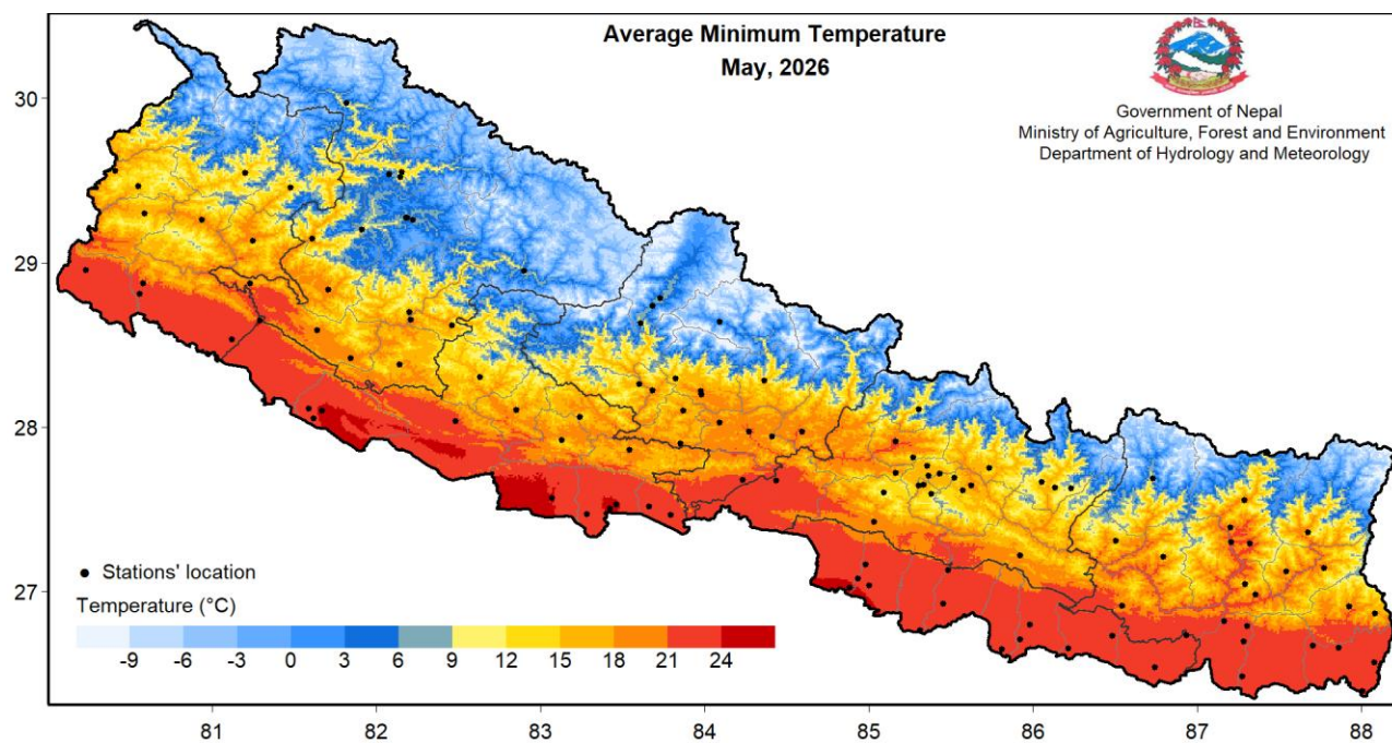
Figure 9: Average Minimum Temperature in May 2026
