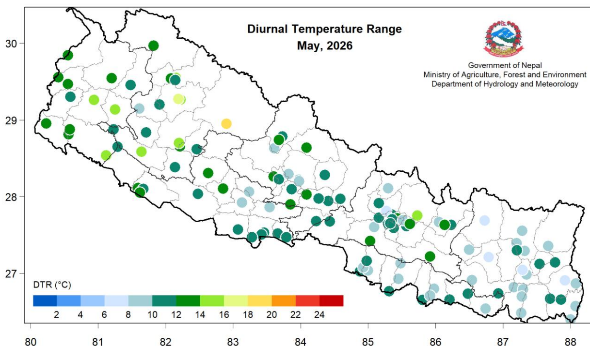
Figure 12: Station plot of diurnal temperature range for May, 2026
