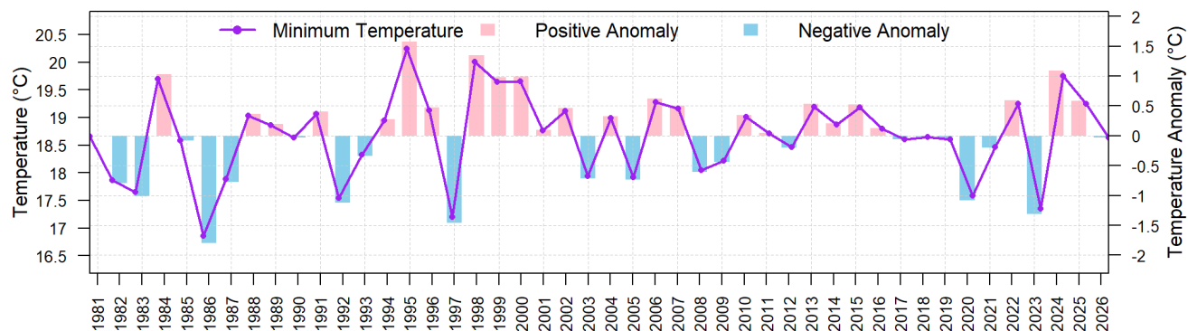
Figure 11: All Nepal monthly average minimum temperature of May from 1981 to 2026 of 64 stations (average of monthly average minimum temperature at stations having long term data)
