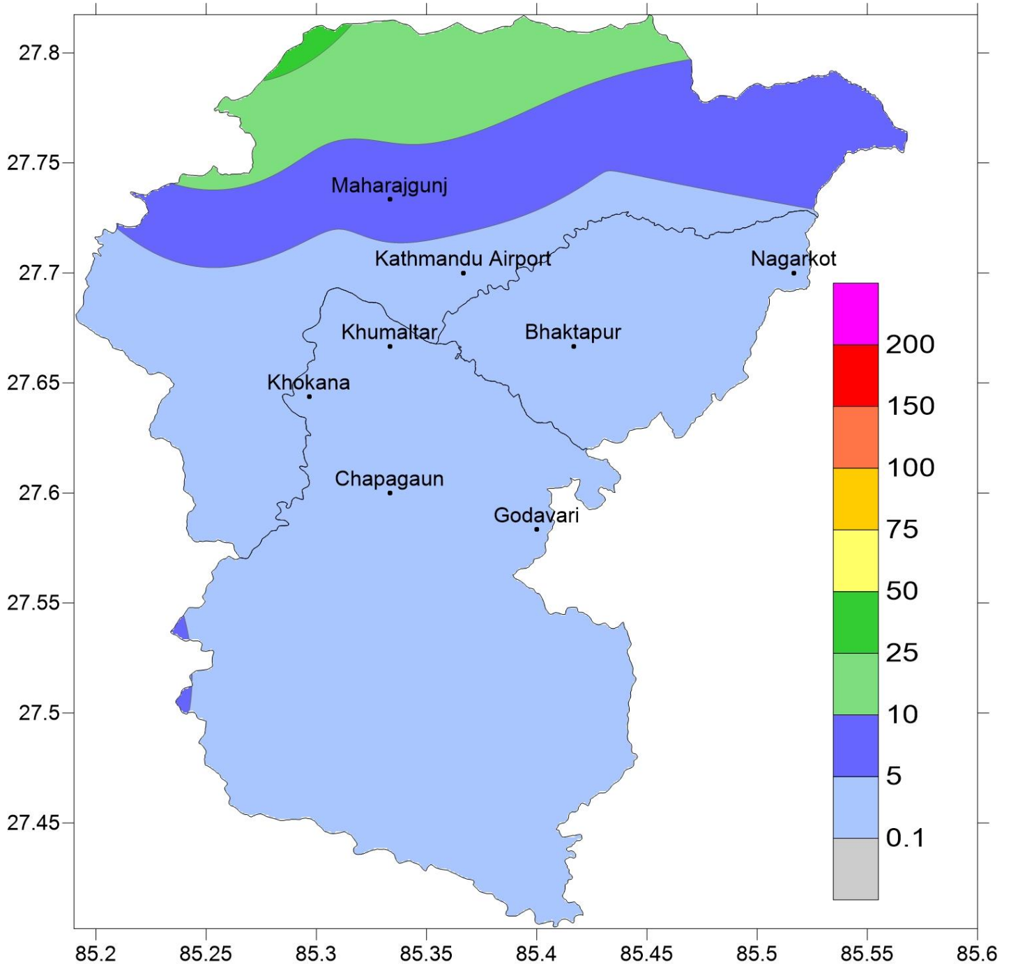
Fig. 1 : Rainfall over various stations in the Kathmandu Valley in mm. (21 st August 2020)
