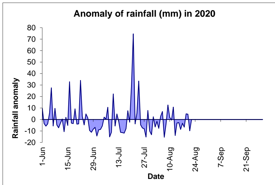
Fig. 3: Anomaly of observed daily averaged rain of 8 stations with daily average of normal of the 8 stations shown in fig. 1 above.
