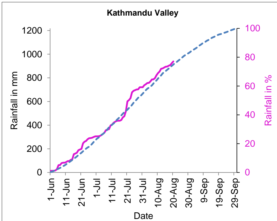
Fig. 2 : In the above graph, blue dashed (---) line indicates the average of daily accumulated normal precipitation of 8 stations during monsoon season (June-September) and pink solid line (—) indicates the average of daily accumulated precipitation of this monsoon. The 8 stations are shown in the fig.1 above.
